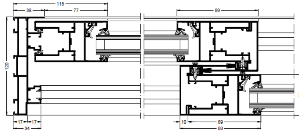
Horizontal section detail through sliding vent
