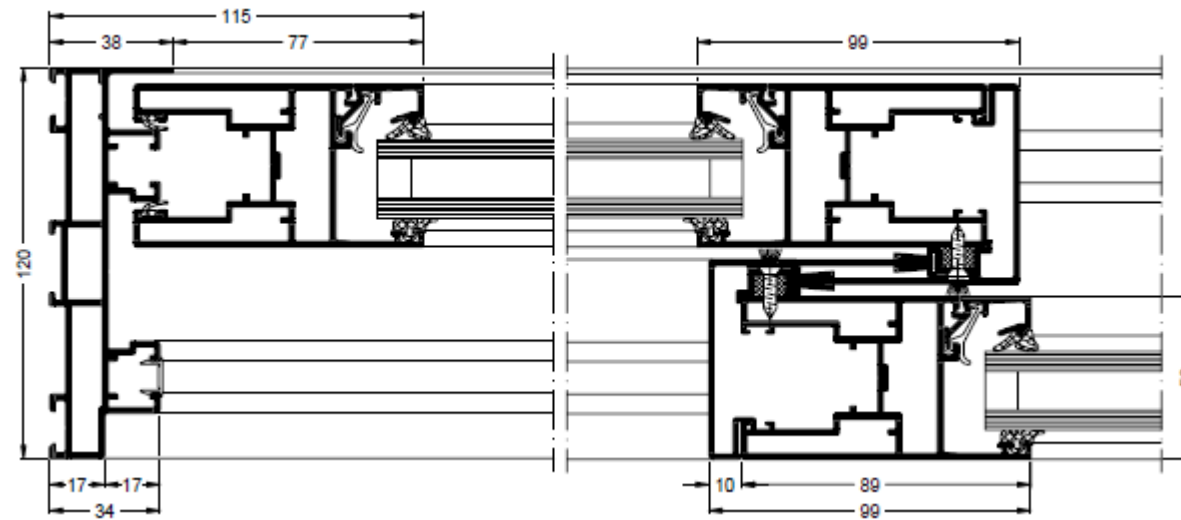
Horizontal section detail through meeting stile
