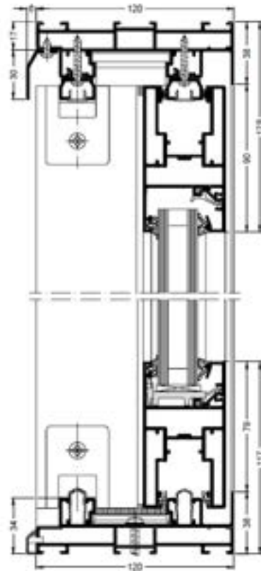
Vertical section detail through sliding vent
