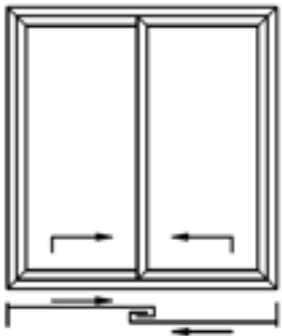
B Lift-and-slide
